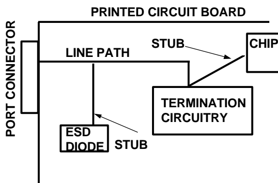
Figure I.1 - Line path definitions
