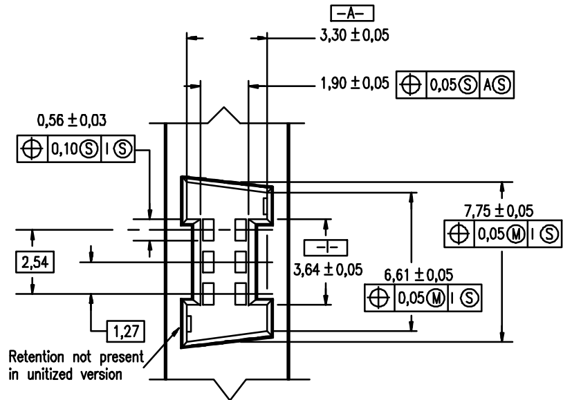
Figure 23 - Internal cable and backplane port connector detail
