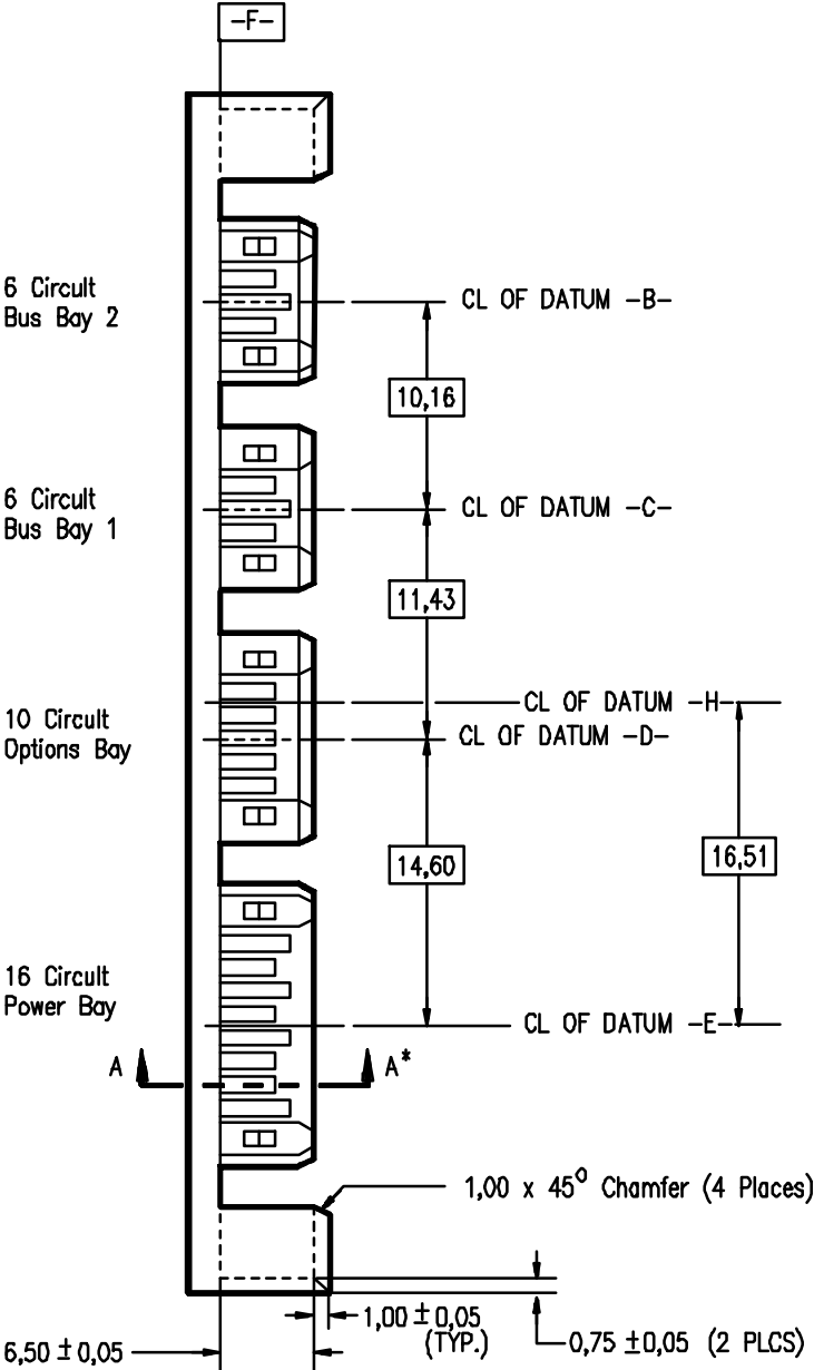
Figure 31 - Internal unitized device connector detail (top view)
