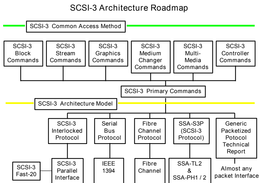
Figure 2 - SCSI-3 Family
