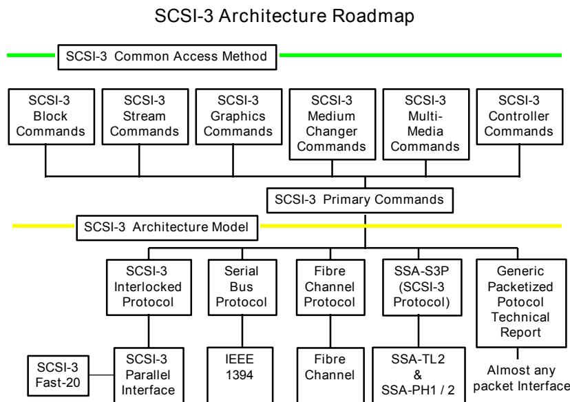
Figure 2 - SCSI-3 Family
