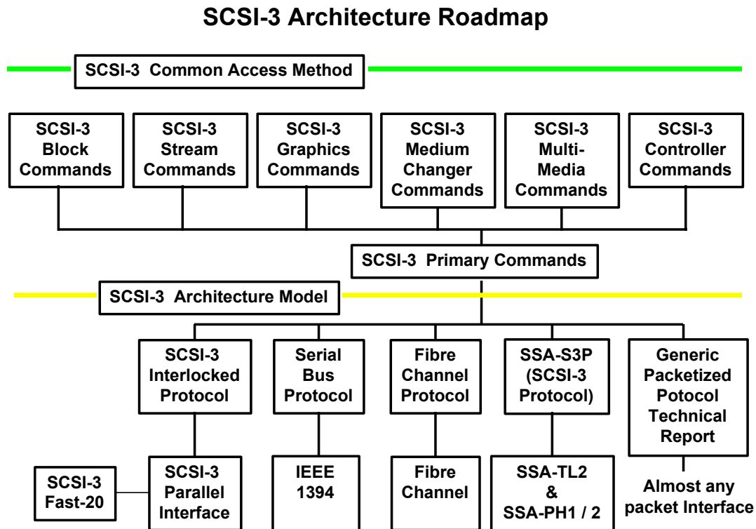
Figure 2 - SCSI-3 Family
