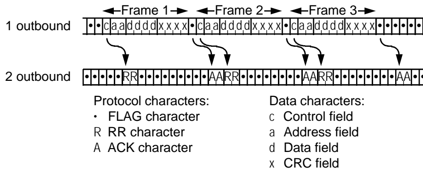
Figure C.1 - Half-duplex transfer
