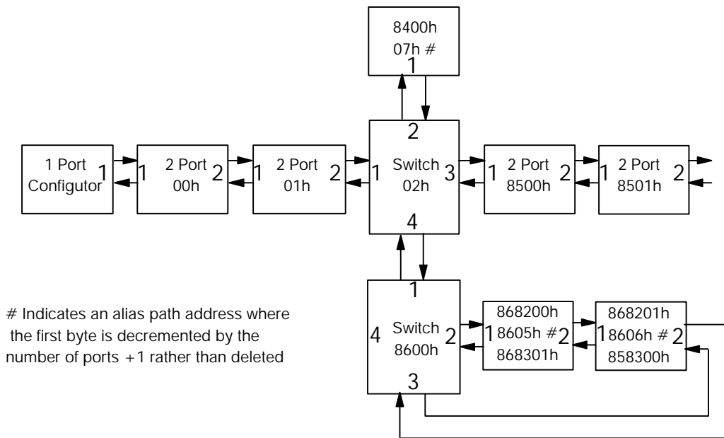
Figure 10 - Path addressing
