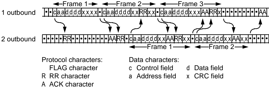
Figure C.2 - Full-duplex transfer
