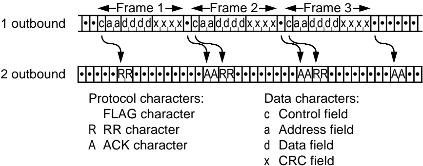
Figure C.1 - Half-duplex transfer
