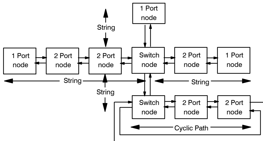
Figure 6 - Complex Web containing a cyclic path
