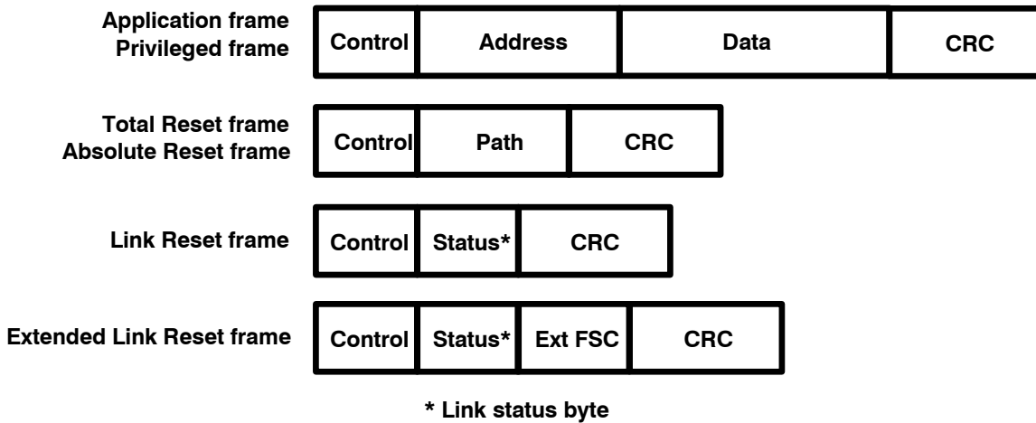
Figure 8 - Specific frame format
