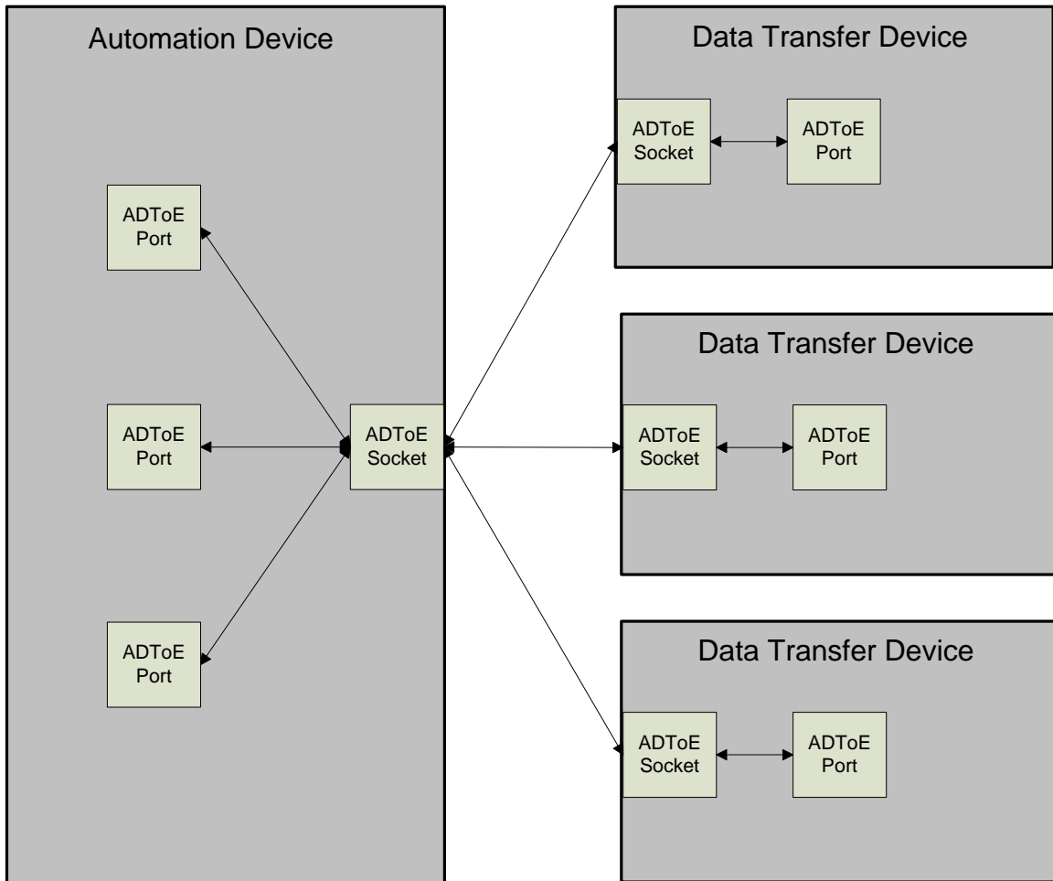
Figure 12 – Example of shared ADToE socket in an automation device
